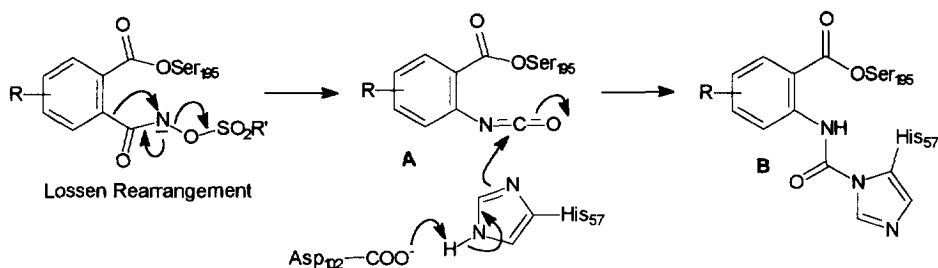
Figure 1. Mechanism of inhibition of serine proteases by 2-[(sulfonyl)oxy]-6-substituted-1 H -isoindole-1,3-diones.
